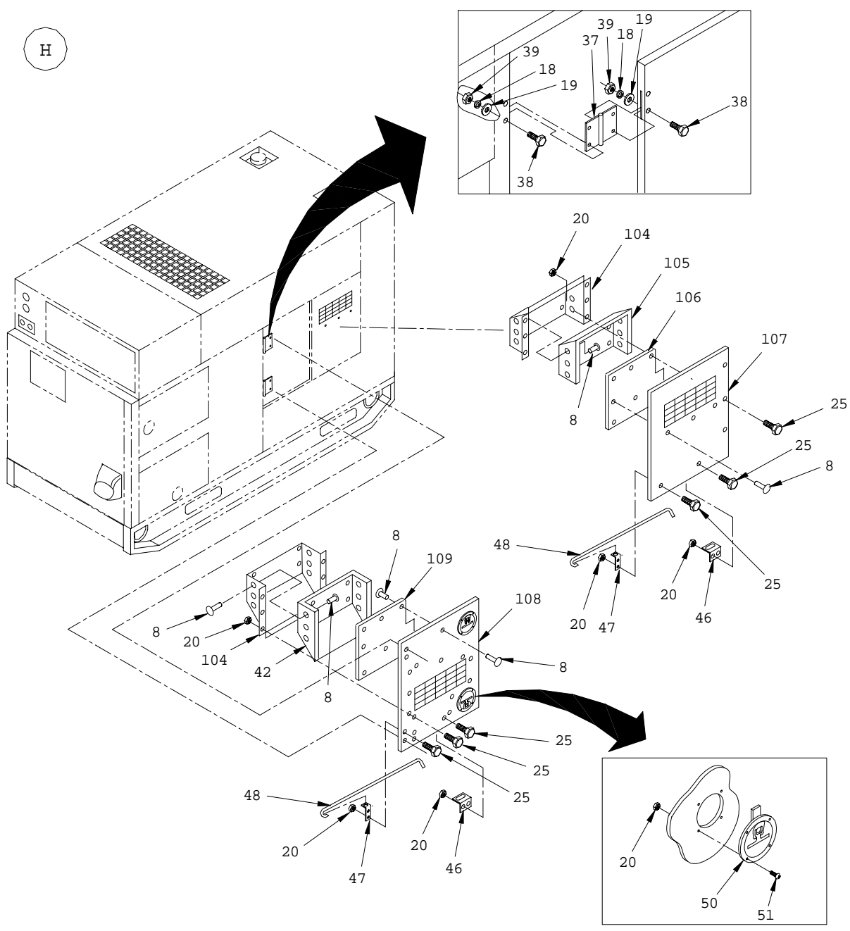
Figure 4. Housing (Sheet 8 of 11)
