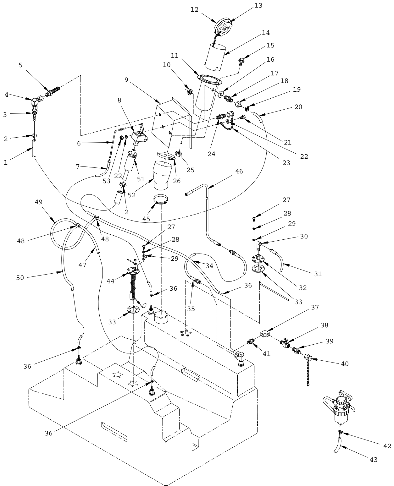
Figure 11. Fuel System (Sheet 1 of 3)
