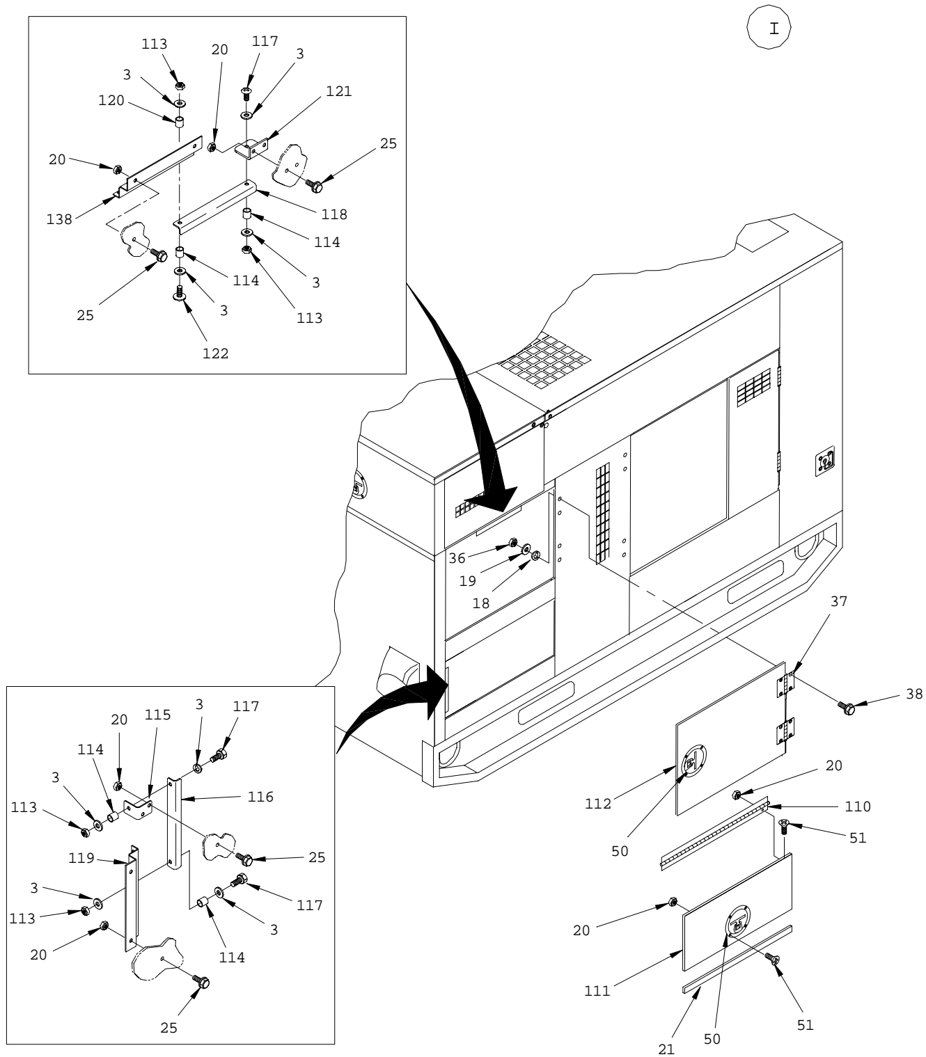
Figure 4. Housing (Sheet 9 of 11)
