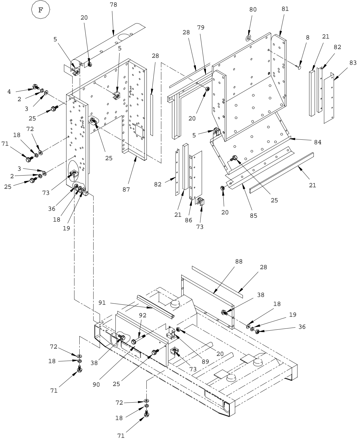
Figure 4. Housing (Sheet 6 of 11)
