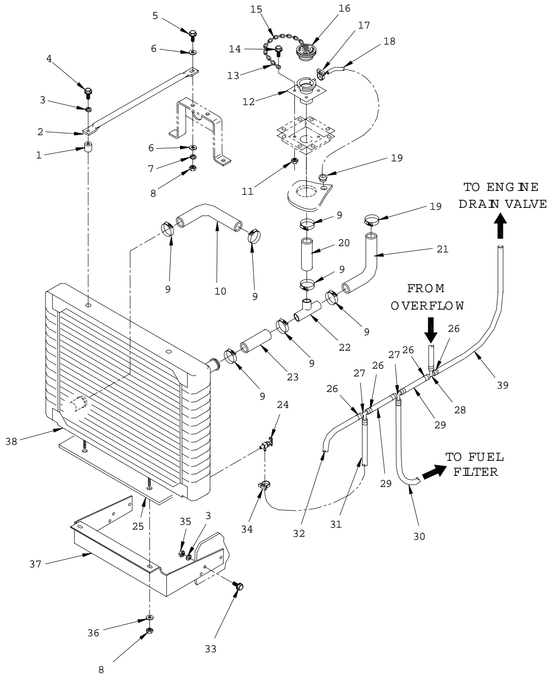
Figure 10. Engine Cooling System (Sheet 1 of 3)
