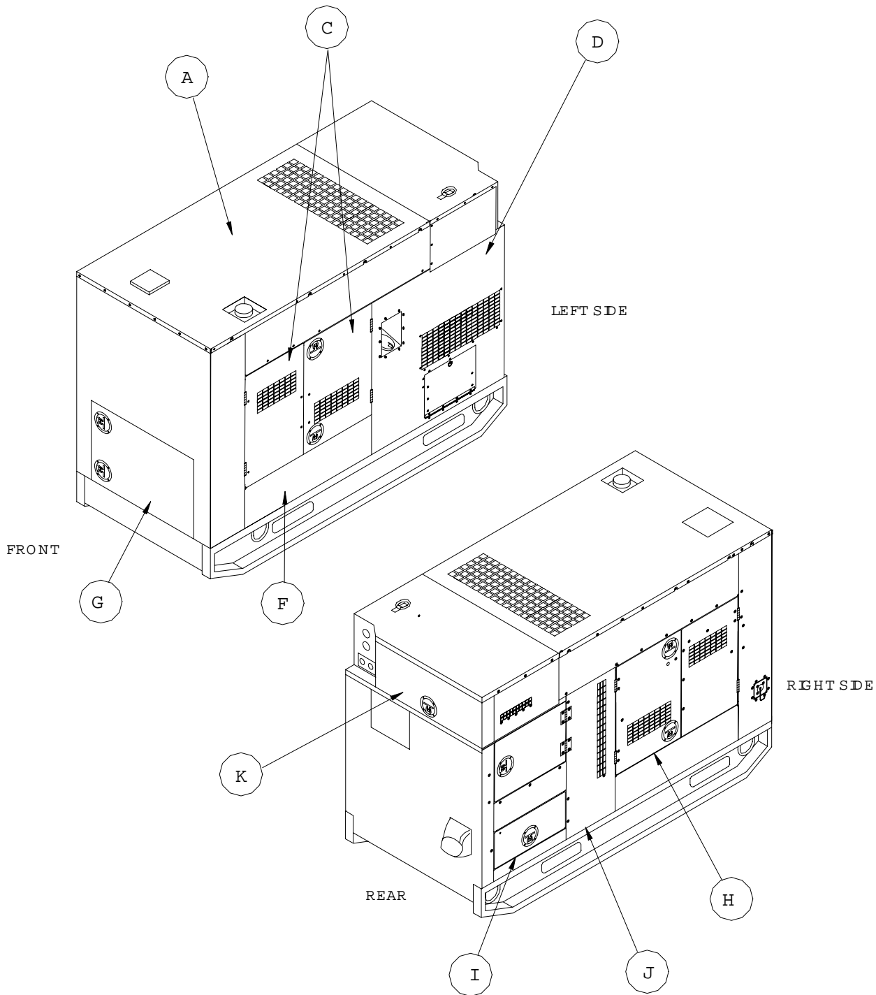
Figure 4. Housing (Sheet 1 of 11)
