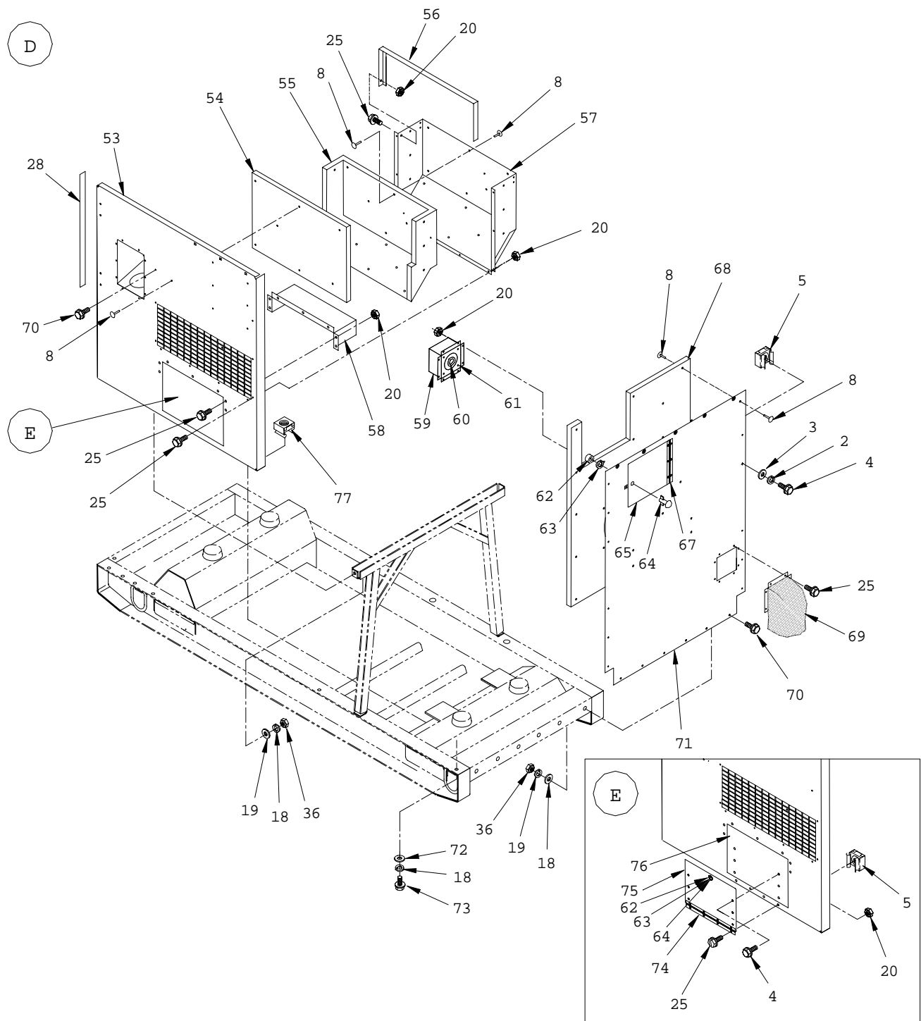
Figure 4. Housing (Sheet 5 of 11)
