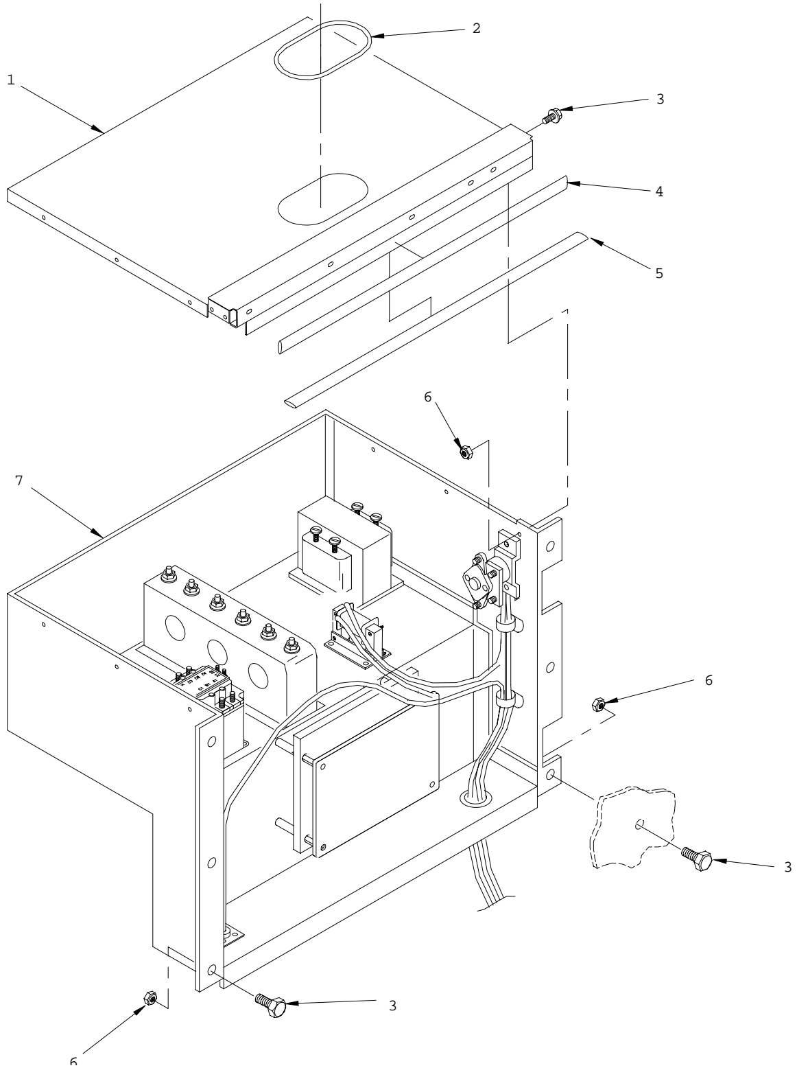
Figure 14. Output Box Assembly (Sheet 1 of 3)
