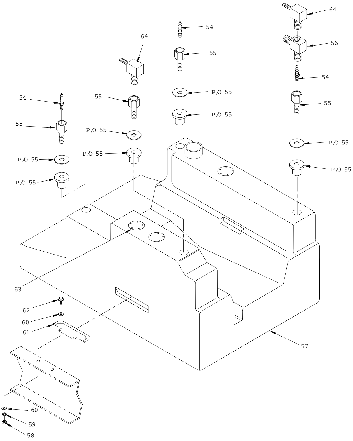
Figure 11. Fuel System (Sheet 2 of 3)
