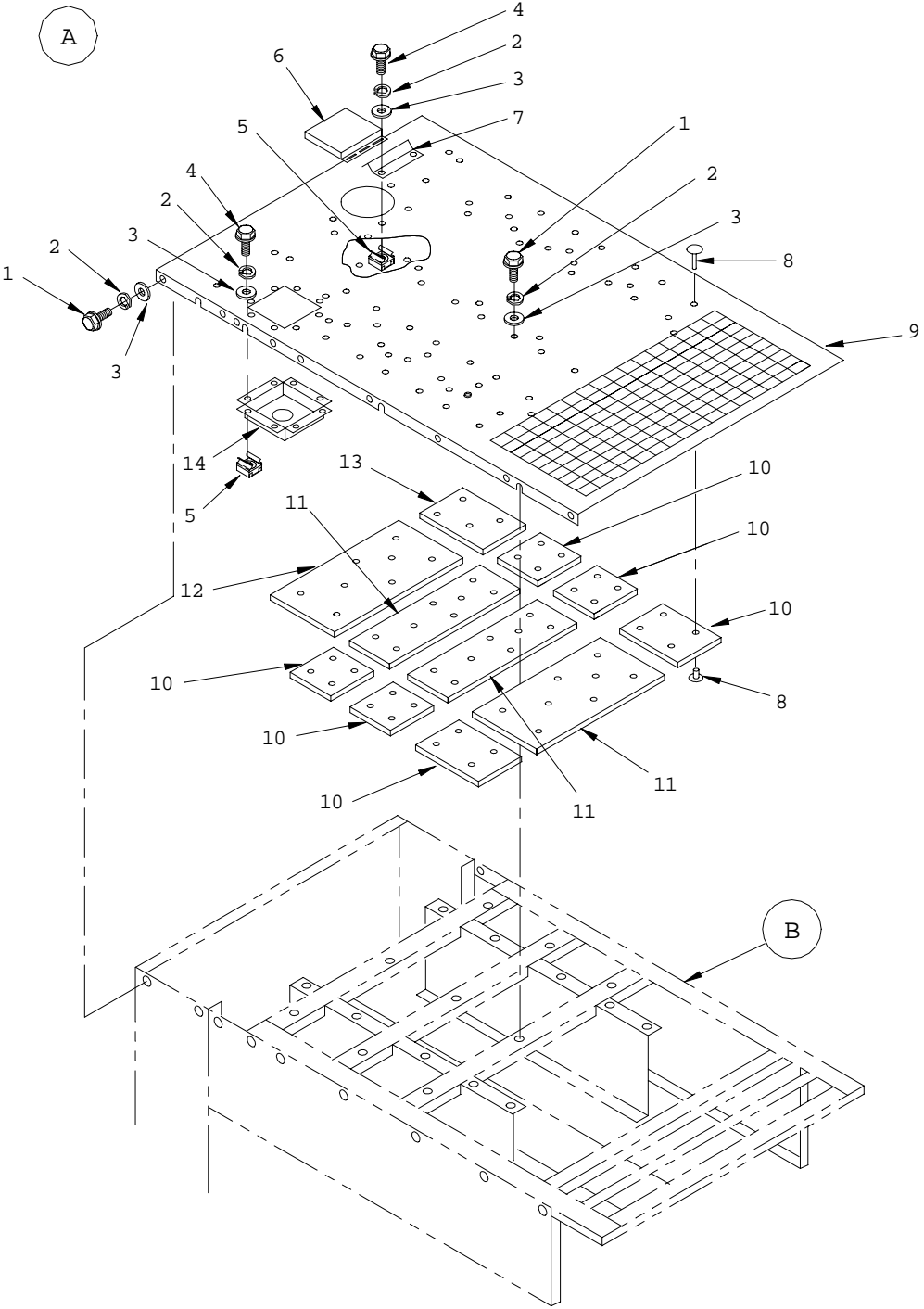
Figure 4. Housing (Sheet 2 of 11)
