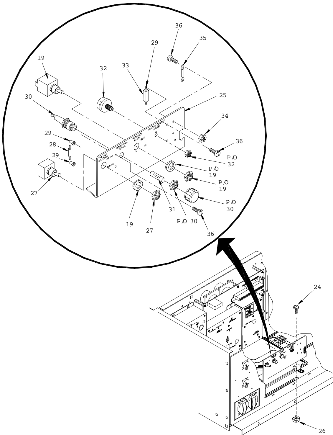
Figure 5. DCS Control Box Assembly (Sheet 5 of 11)
