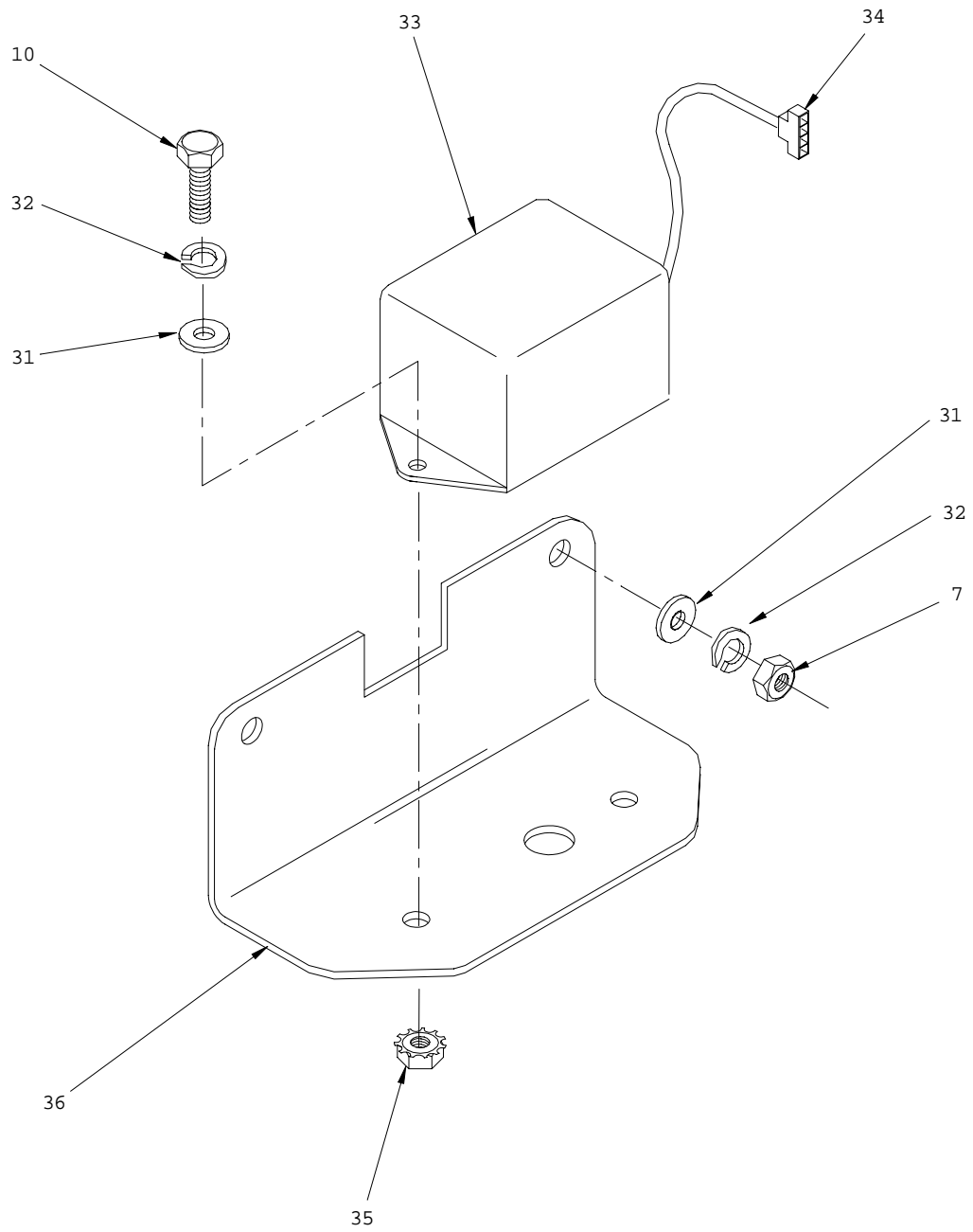
Figure 19. Engine Accessories (Sheet 4 of 4)
