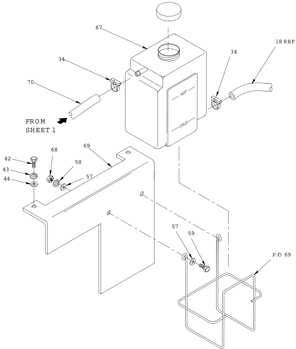
Figure 10. Engine Cooling System (Sheet 3 of 3)
