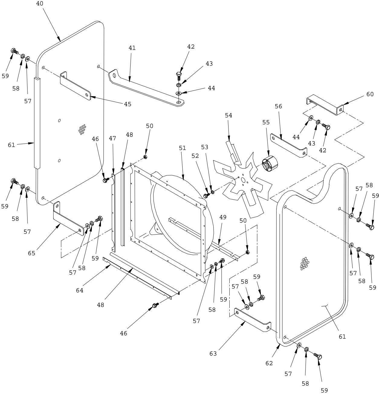
Figure 10. Engine Cooling System (Sheet 2 of 3)
